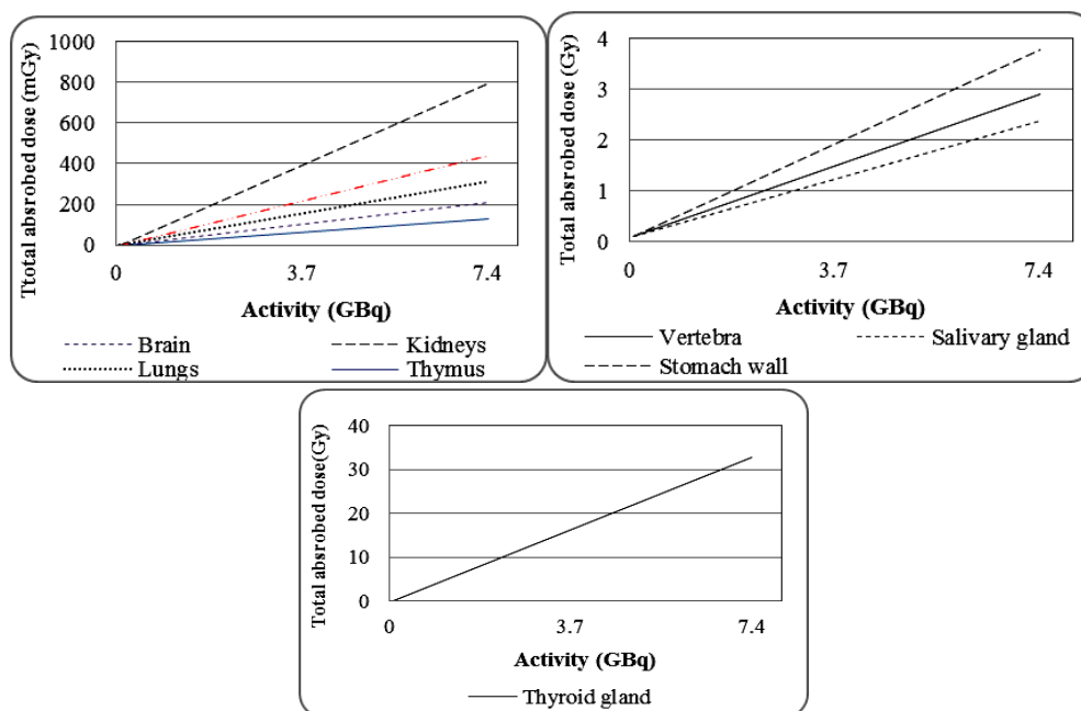
Fig. 4. Total absorbed dose of critical organs against administrated activity for: (a) Brain, lungs, heart walls, thymus and kidneys (b) Salivary glands, stomach walls, and cervical vertebra (c) Thyroid gland
