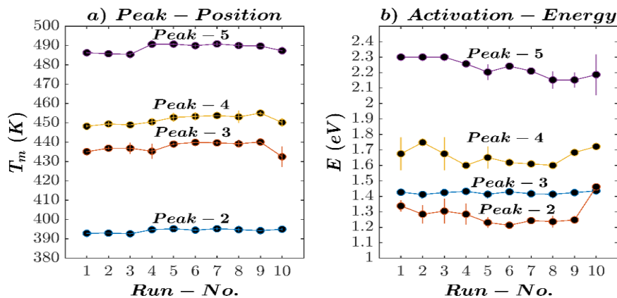
Fig. 7. Peak Position and activation energy values for the low-temperature glow-peaks of sensitized LiF dosimeters readout under the same temperature readout range [323-633] K for 10 times.
