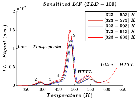
Fig. 1. Effect of different temperature readout ranges on sensitized TLD-100 dosimeters.
