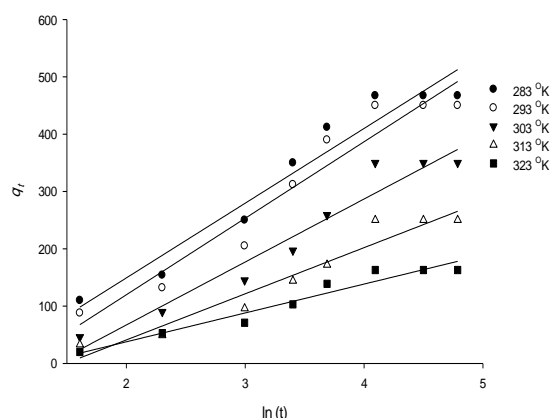
Figure 11: Elovich adsorption model of AR 141 on MNPs at different temperatures. ( C_{\text{dye}} = 80 ppm, pH = 3.0, adsorbent dose = 200.0 mg)
