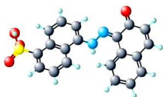
Figure 1. Molecular structure of 3D Conformer of Parent Acid Red 141 (AR141)
