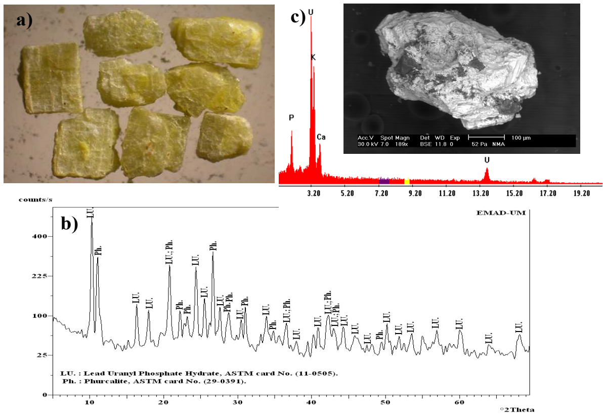
Fig. 10: Stereophotograph of phurcalite grains separated from El Sela sheared granite tailed with ESEM spectrograph and XRD diffractogram.
