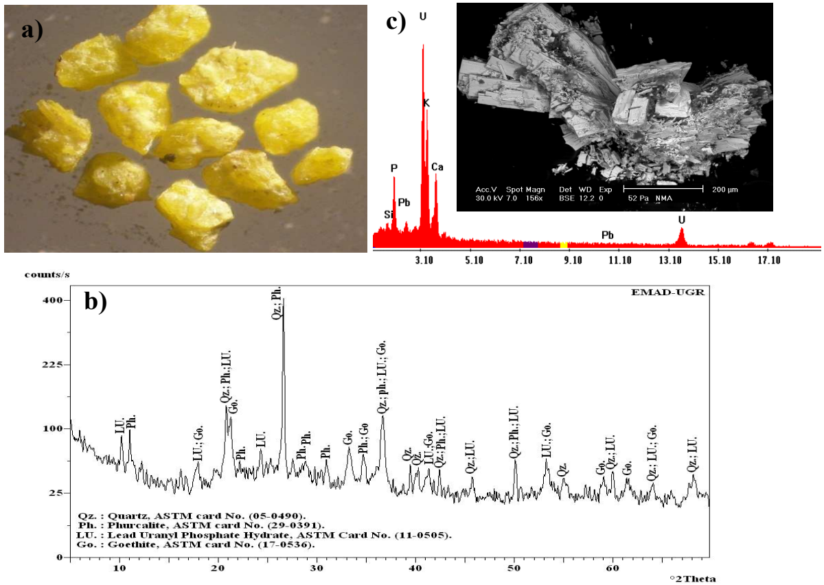
Fig. 9: Stereophotograph of lead-metautinite grains separated from El Sela sheared granite tailed with ESEM spectrograph and XRD diffractogram.
