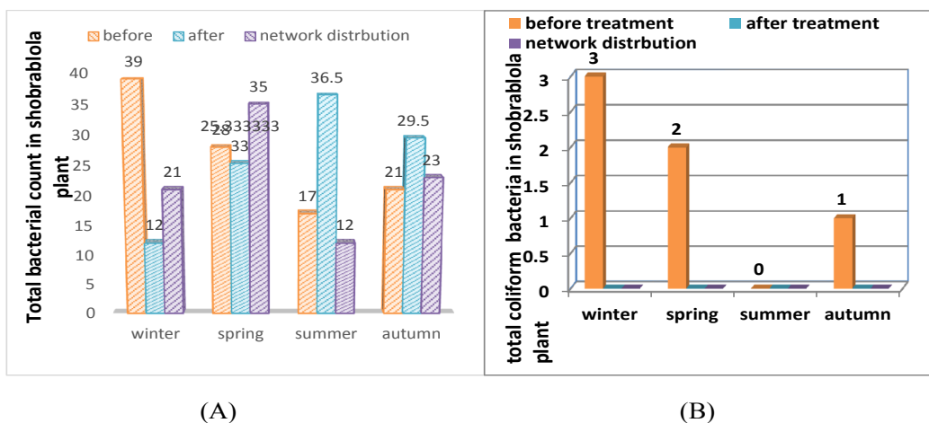
Figure (2) Relationship between total bacterial count (A) and total Coliform bacteria(B) (before, after treatment and network distribution) seasonal variation of shobra-blola plant.
