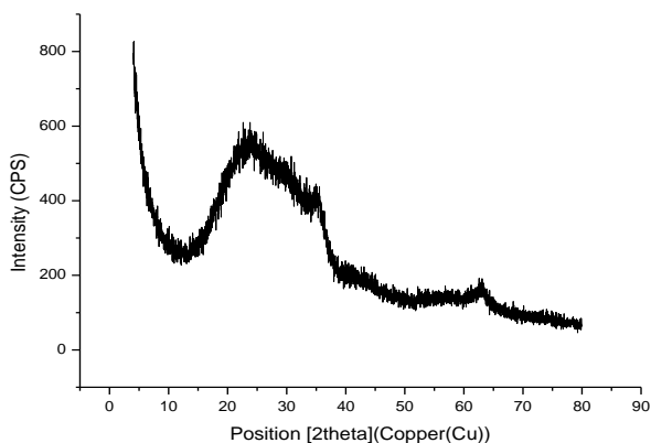
Fig. 4: XRD of \alpha - Fe 2 O 3 thin film prepared by flame spray of precursor followed by thermal- induced oxidative decomposition at 250°C of precursor thin film on glass slide.
