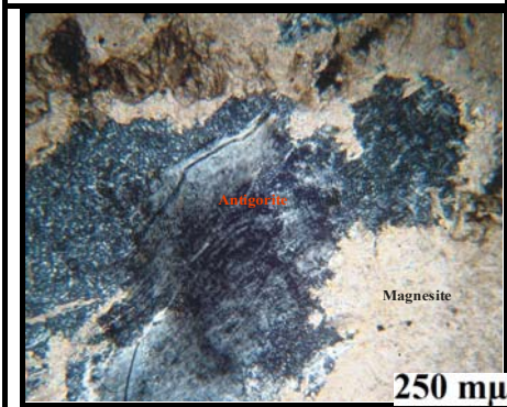
Fig.16: Photomicrograph showing antigorite and magnesite crystals (CN).
