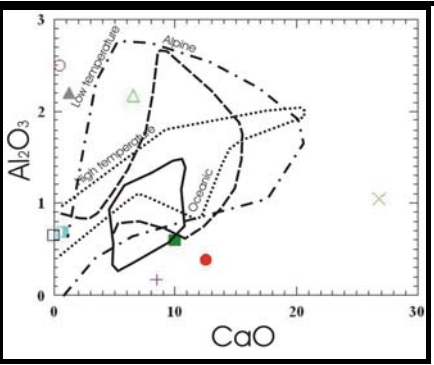
Fig.40: Al 2 O 3 -CaO binary diagram for the talc-carbonate (Aumento and Laubart, 1971). Legend as in Fig. (24).
