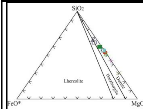
Fig.25: SiO 2 -FeO* MgO ternary diagram for talc-carbonates (Pfeifer, 1979). Legend as in Fig. (24).
