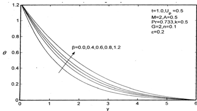
Fig.(2): Temperature profiles against y for different values of thermal dispersion \beta .
