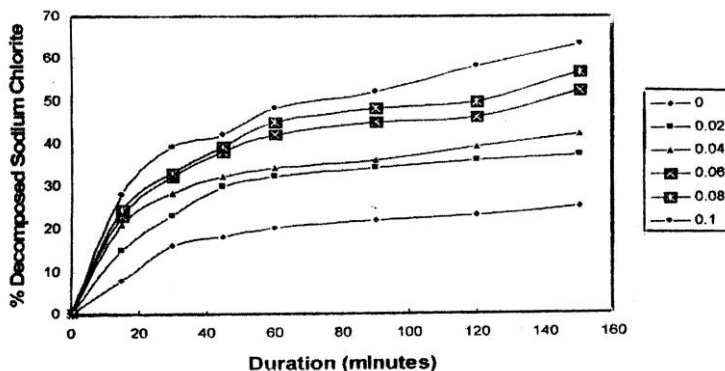
Fig. 1: Effect of [HMTA] on NaClO 2 Decomposition Reaction Conditions: Temperature 95°C, Sodium Chlorite 2g/l.
