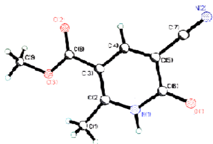
Fig. (2): X-ray crystallography of Methyl 5-cyano-2-methyl-6-oxo-1,6-dihydropyridine-3-carboxylate 11 .
